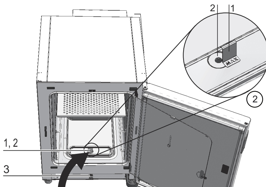
Figure 3-13. Water Reservoir
