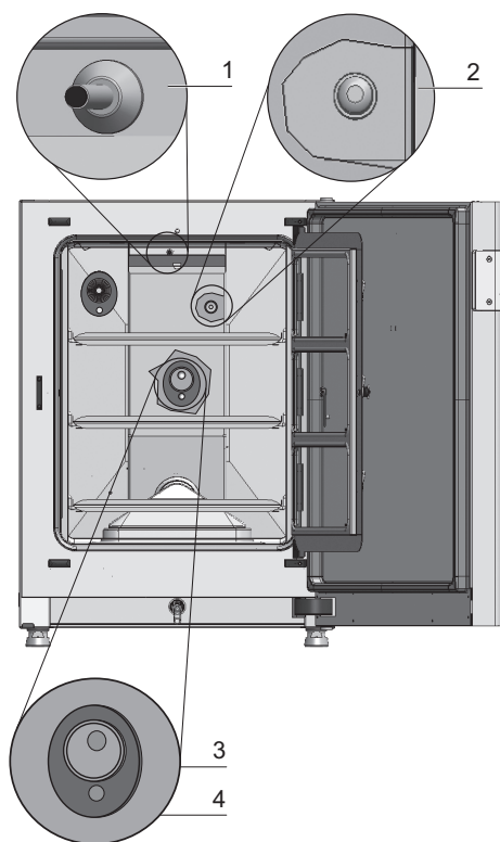
Figure 3-7. Temperature, O 2 , CO 2 and Humidity Sensors
