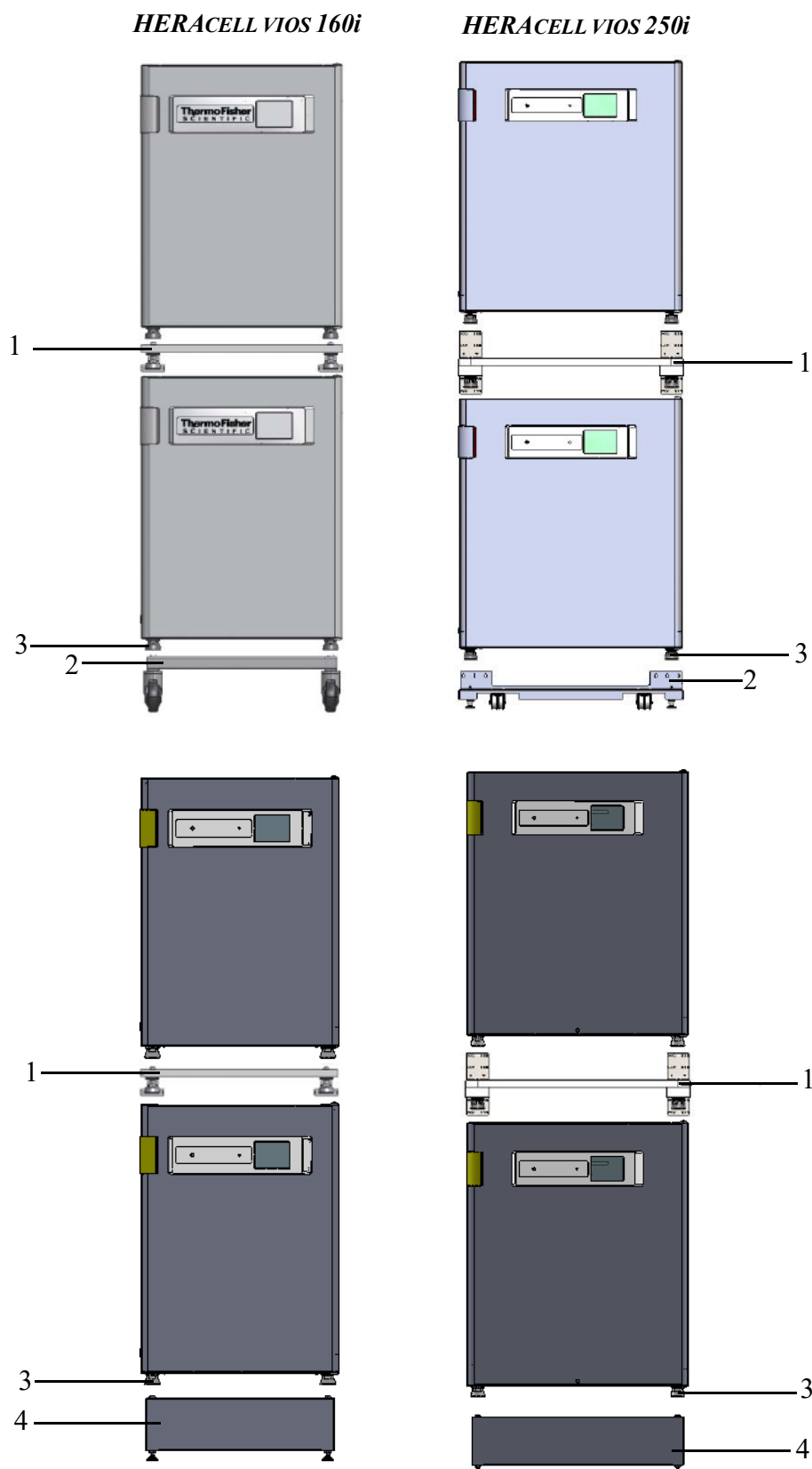
Figure 2-3. Stacking
